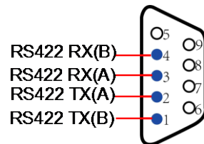
For RS422 Mode
